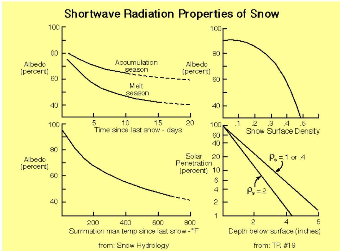
Figure A-4. Shortwave radiation properties of snow.
