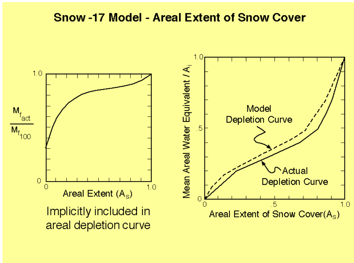
Figure 9. Effect of changing melt rates on the areal depletion curve.
