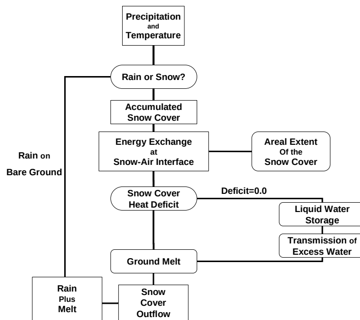
Figure 1. Flowchart of the SNOW-17 model
