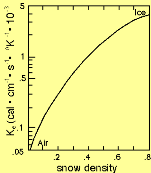
Figure A-6. Variation in effective thermal conductivity with density.
