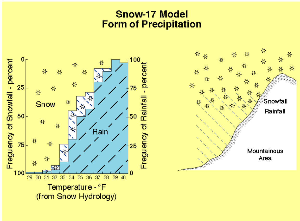
Figure 2. Variation of form of precipitation with temperature and elevation.
