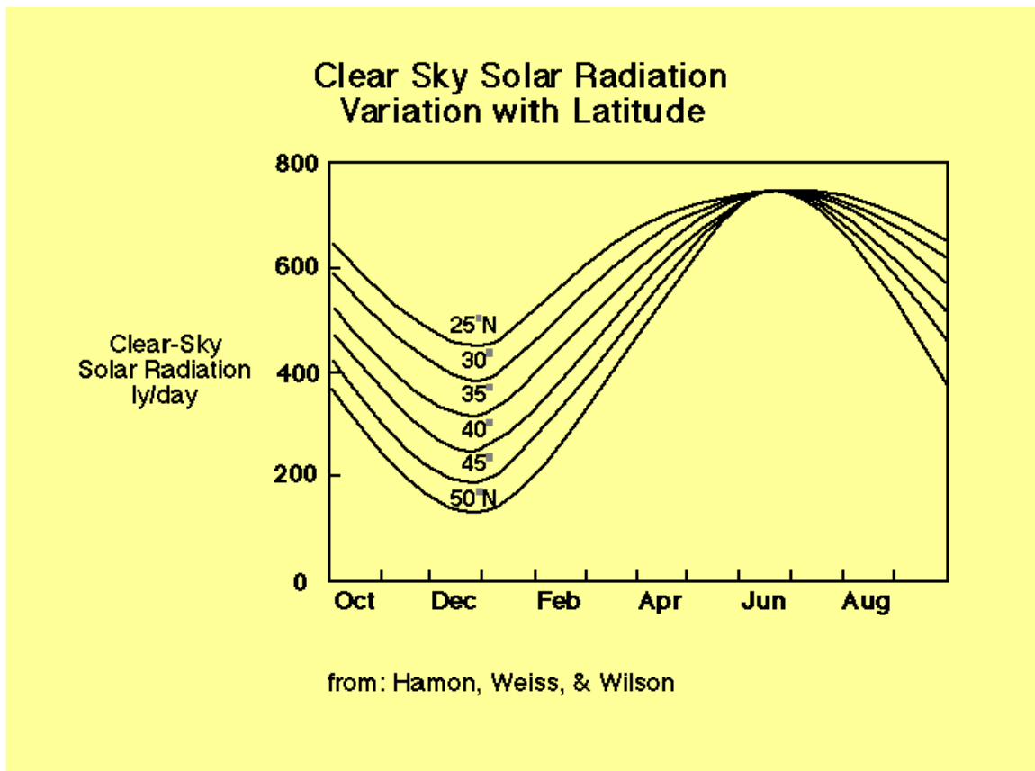
Figure A-2. Variation of clear sky solar radiation with time of year and latitude.
