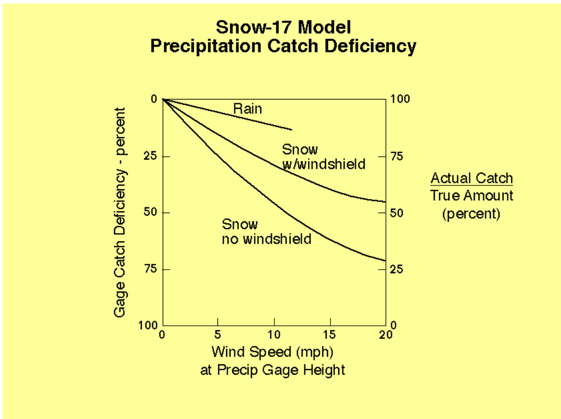
Figure 3. Effect of wind on precipitation catch.
