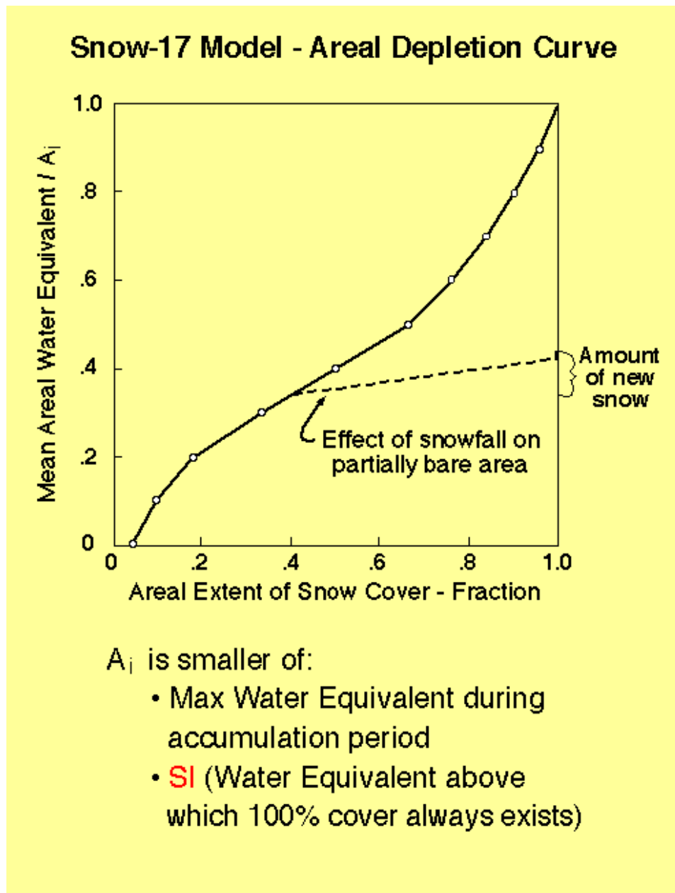
Figure 8. SNOW-17 areal depletion curve.
