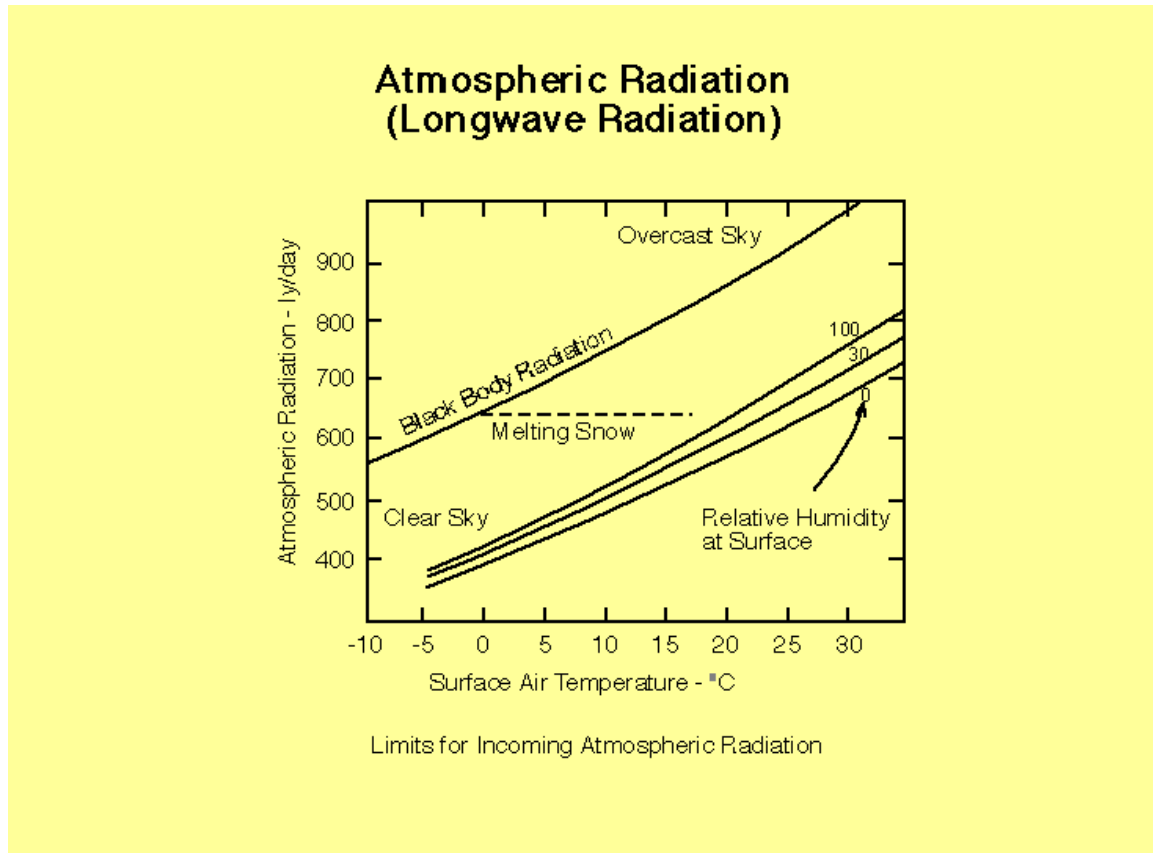
Figure A-5. Atmospheric radiation as a function of temperature and sky conditions.
