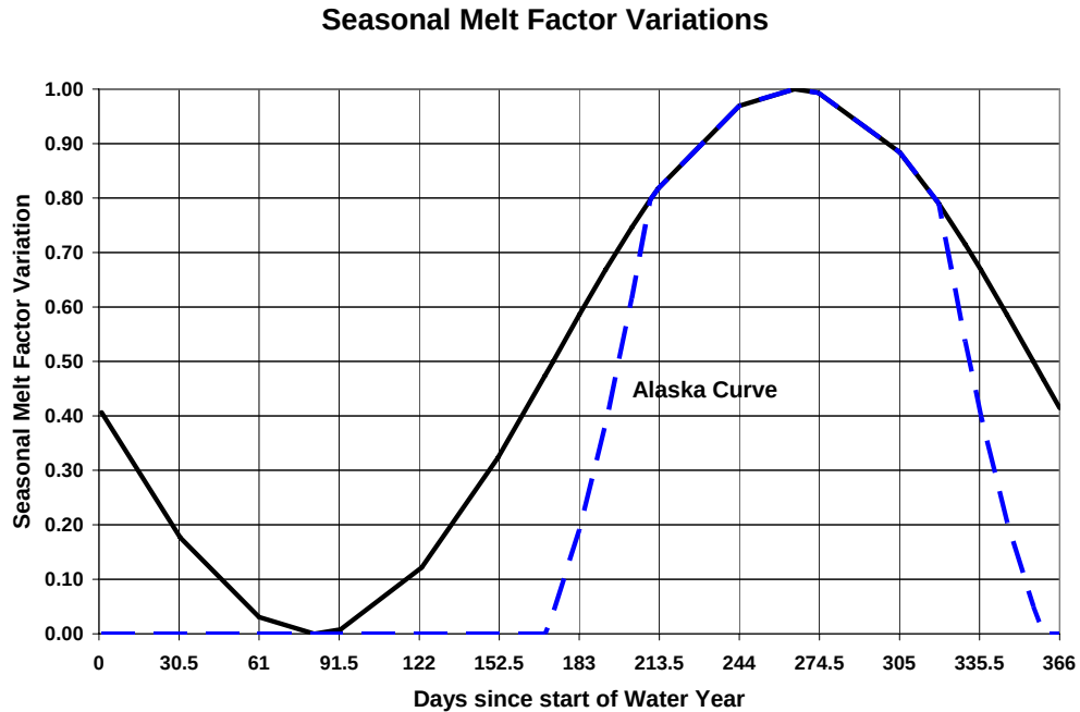
Figure 5. Seasonal melt factor variations used by SNOW-17.
