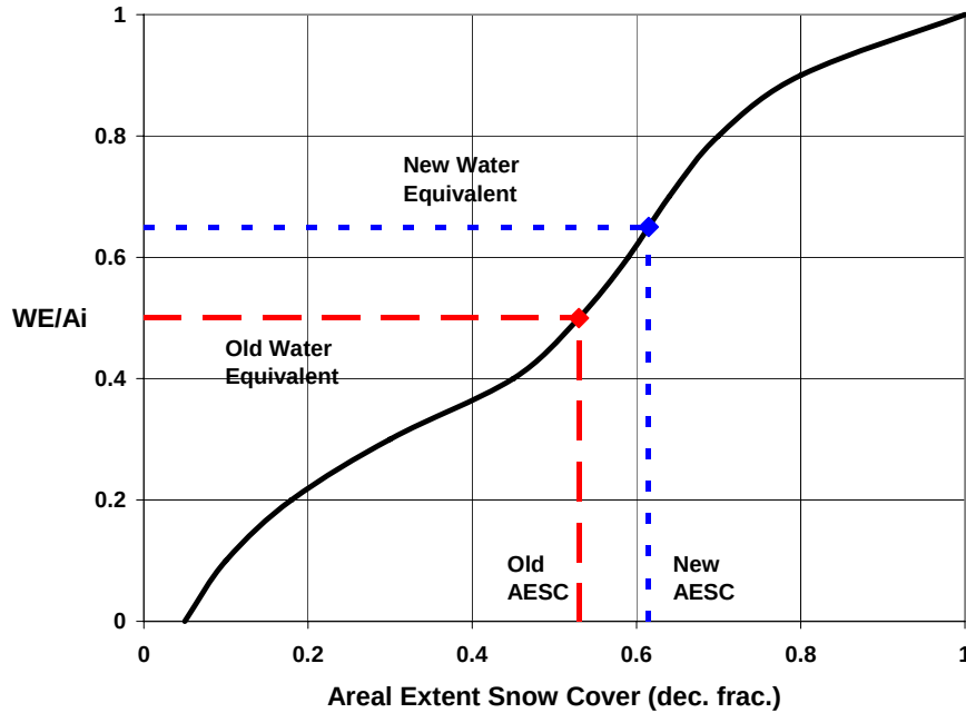
Figure 10. Effect of changing water equivalent on the areal extent of snow cover.
