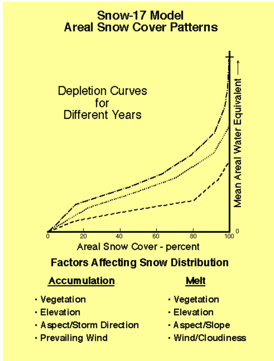
Figure 7. Variation in Depletion Curves from year to year.
