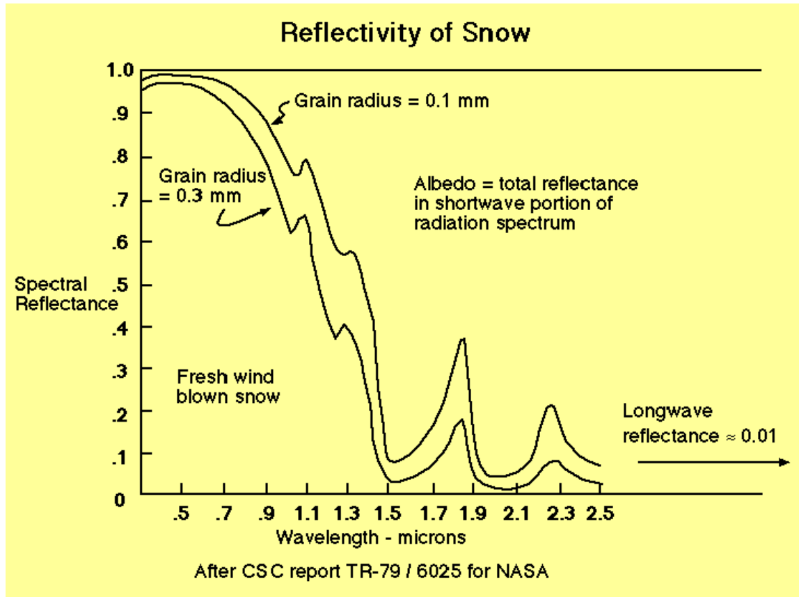
Figure A-3. Variation in reflectivity of snow as a function of wave length.
