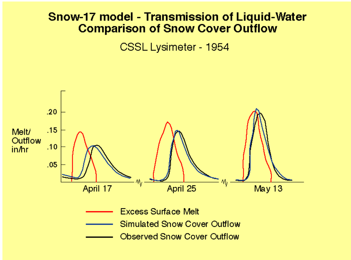
Figure 6. Verification of liquid water transmission algorithms.
