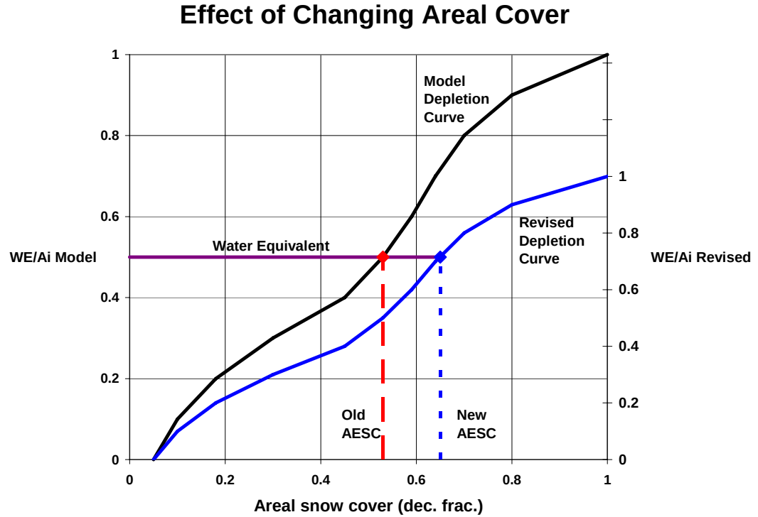
Figure 11. Effect of changing areal snow cover on the depletion curve.
