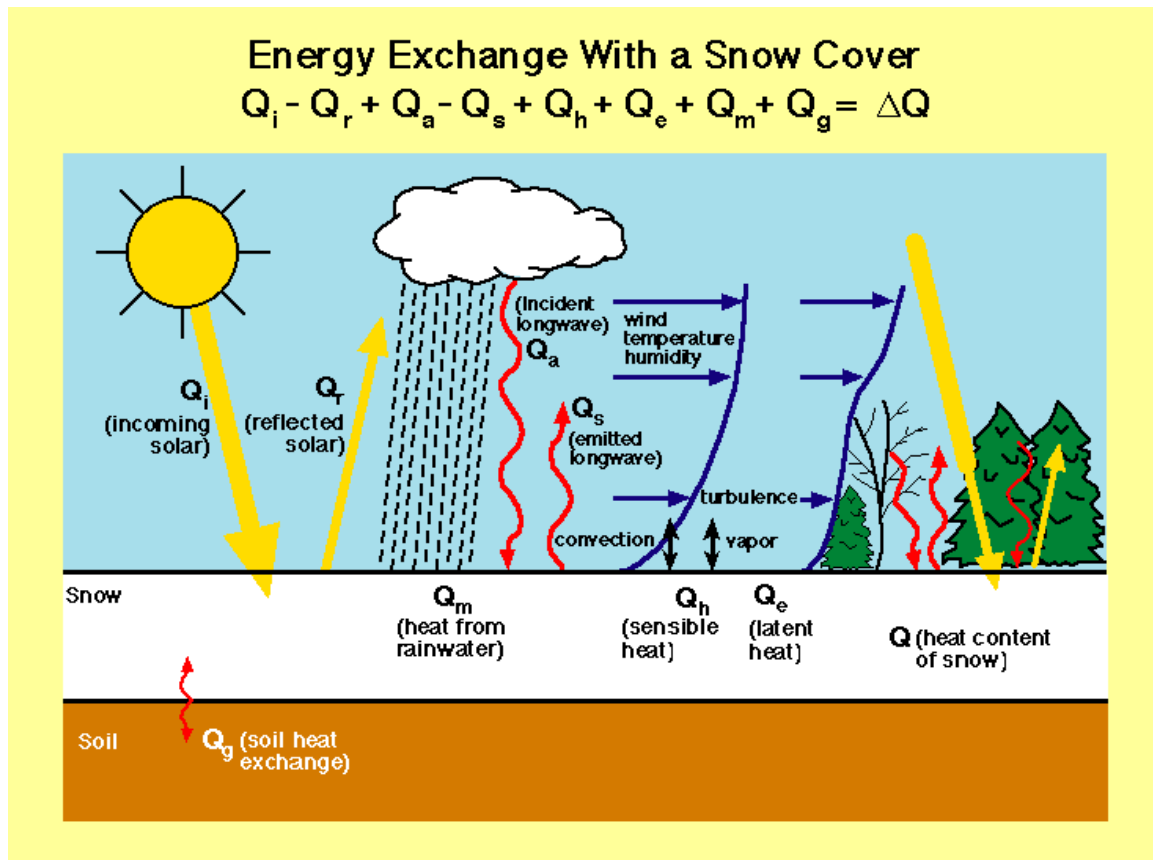
Figure A-1. Summary of snow cover energy exchange
